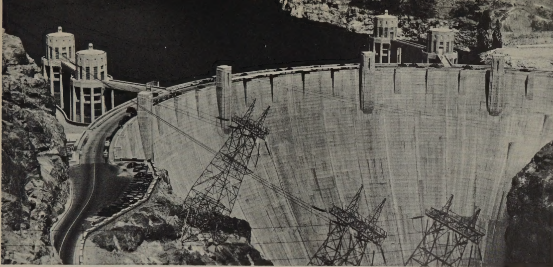
Pioneer of Reclamation's great multipurpose projects, Hoover Dam is still the highest dam in the Western Hemisphere.
